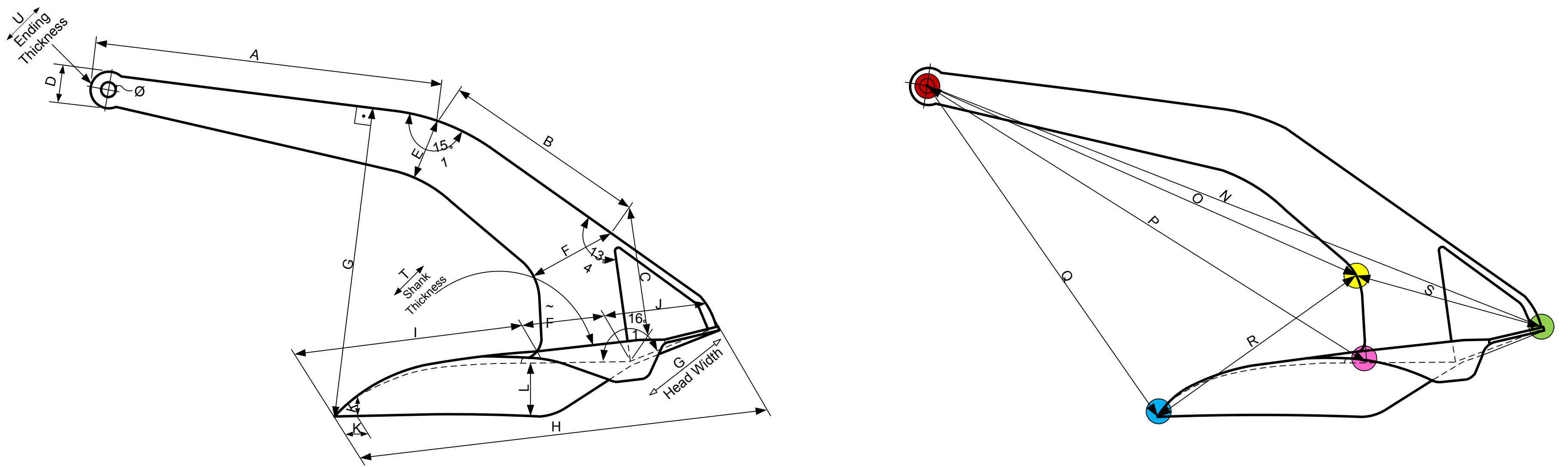
ULTRAnchor Template Dimensions (mm)
